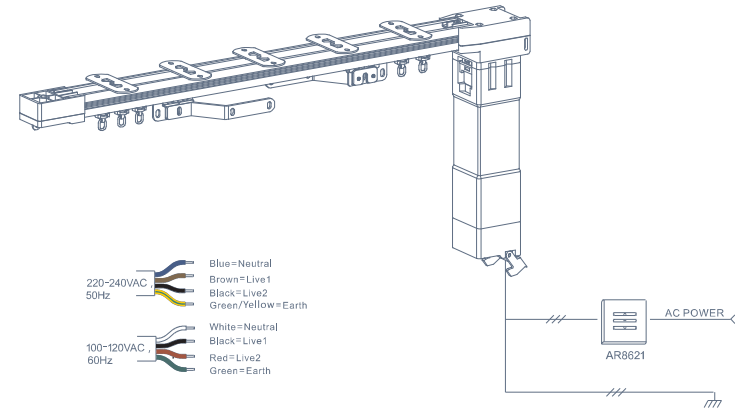
Single track system with single open on drapery blind
